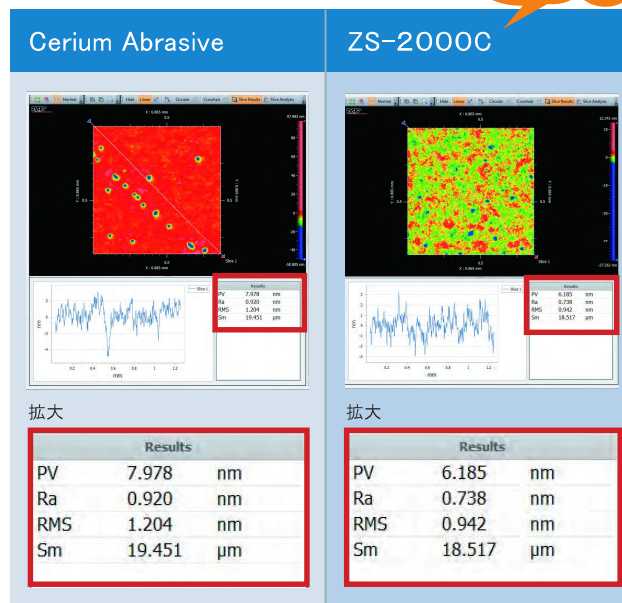
Comparison of Surface Roughness (using LP66 Pad)
